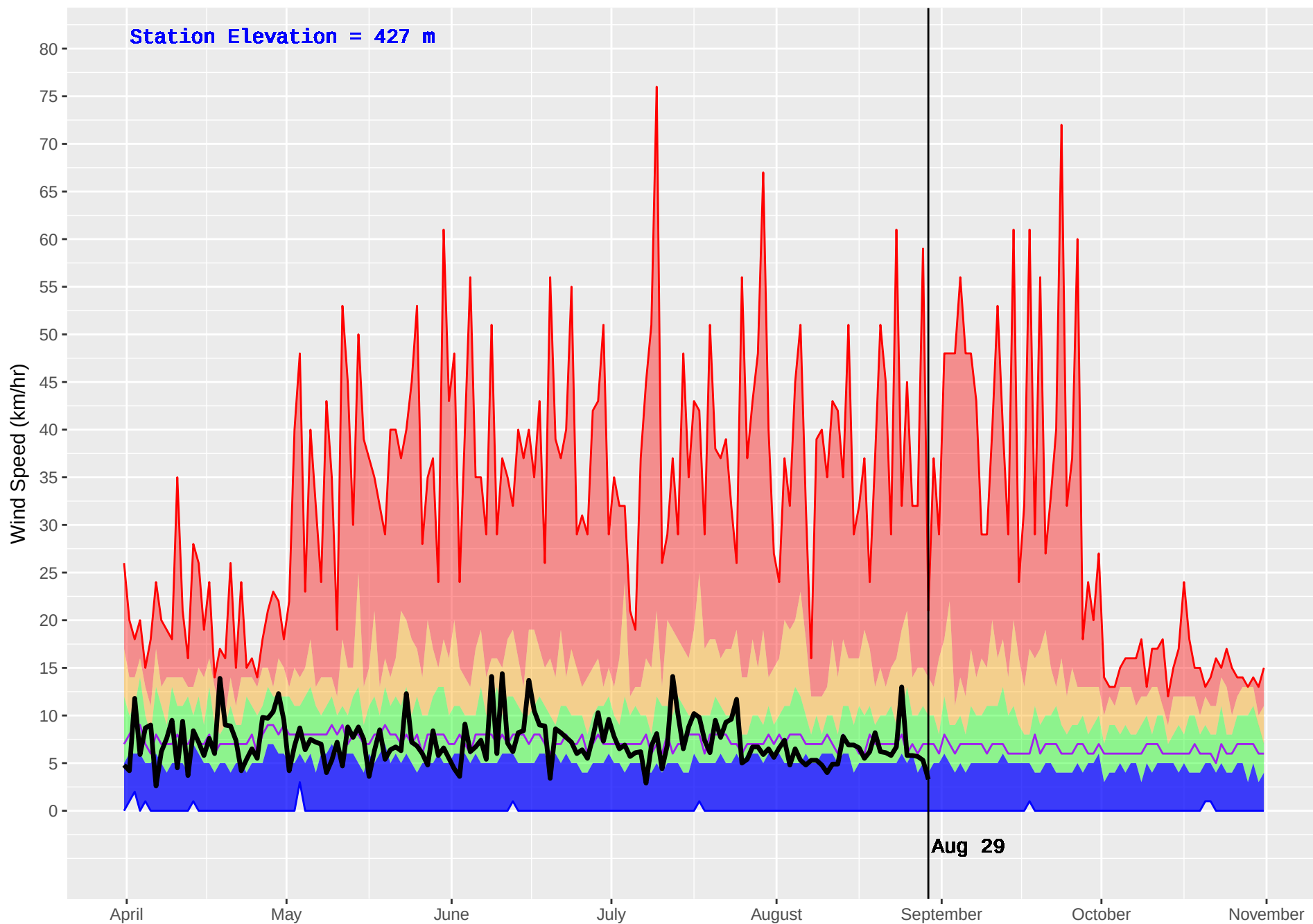
PENTICTON RS (328) : Historical (1970–2016) and Current (2017) Noon Wind Speed
